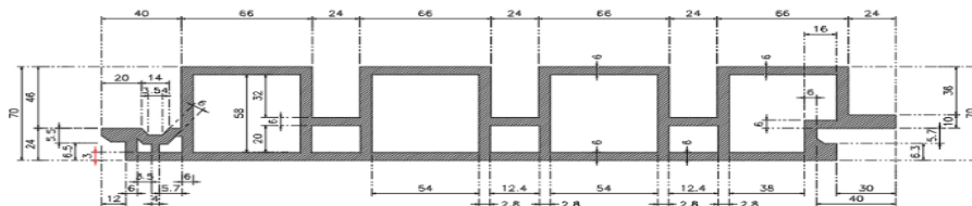
WPO18035 Profile Drawing Detail
