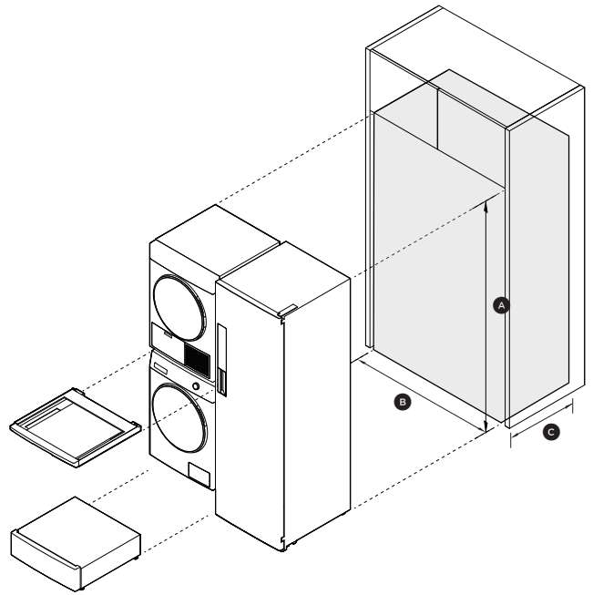
ISO VIEW
