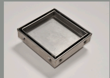
Premium Tile Insert Drain Suits tiles up to 12mm 130mm x 130mm 23mm Deep DN50
