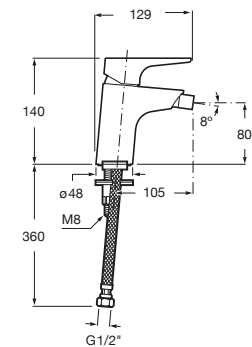
Atlas Bidet Mixer
