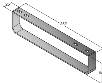
Meridian Wall Basin Side Towel Rail
