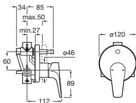
Atlas Shower Mixer with Diverter
