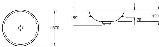
Inspira Round Semi Inset Basin 370
