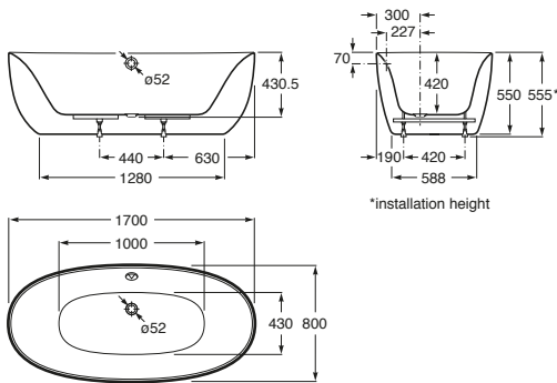
Virginia Freestanding Bath
