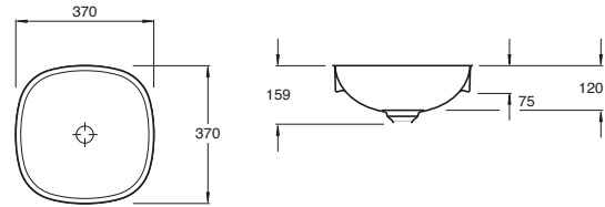
Inspira Soft Semi Inset Basin 370
