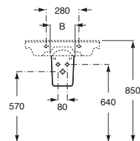
Debba Semi Pedestal to suit Debba Wall Basin 500
