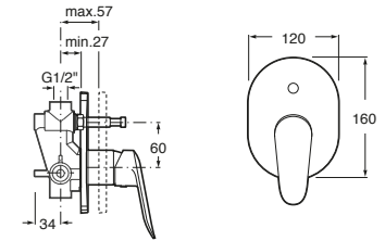
Logica-N Shower Mixer with Diverter
