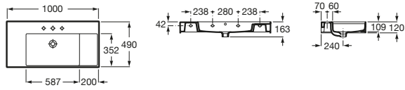
Inspira Wall Basin 1000
