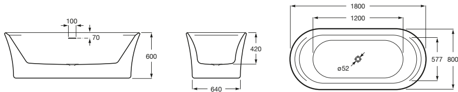
Inspira Freestanding Bath
