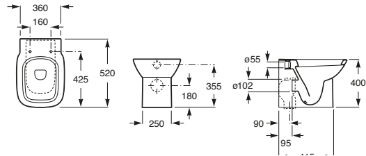
Debba Back to Wall Pan
