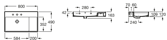
Inspira Wall Basin 800
