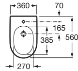
Meridian Wall Hung Bidette 560
