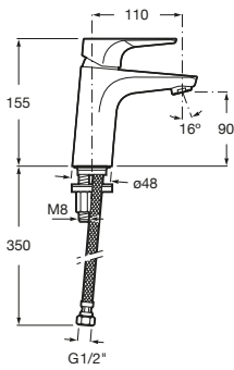
Atlas Basin Mixer
