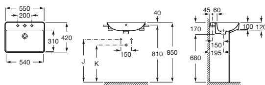
Inspira Square Semi Recessed Basin 550
