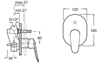
Logica-N Shower Mixer with Diverter
