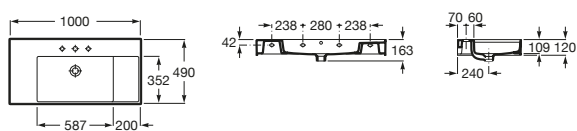
Inspira Wall Basin 1000
