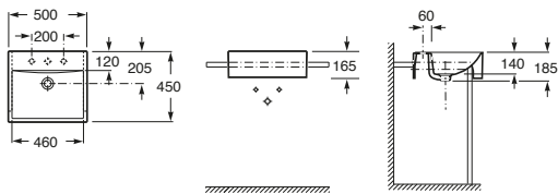
Diverta Semi Recessed Basin 500
