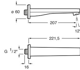
Escuadra Wall Bath Outlet with Diverter
