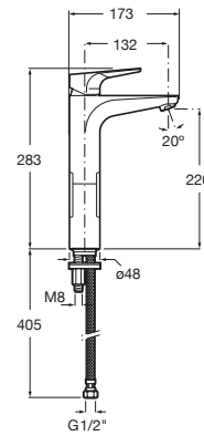
Atlas Extended Basin Mixer
