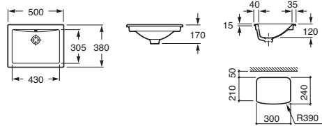
Diverta Inset Basin 500
