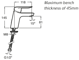
Logica-N Basin Mixer
