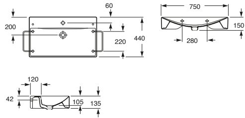
Diverta Wall/Counter Basin 750
