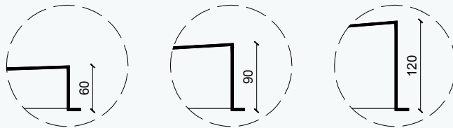
TEGO® PRODUCT CODE TEGO® VOS60L TEGO®VOS90L TEGO®VOS120L
