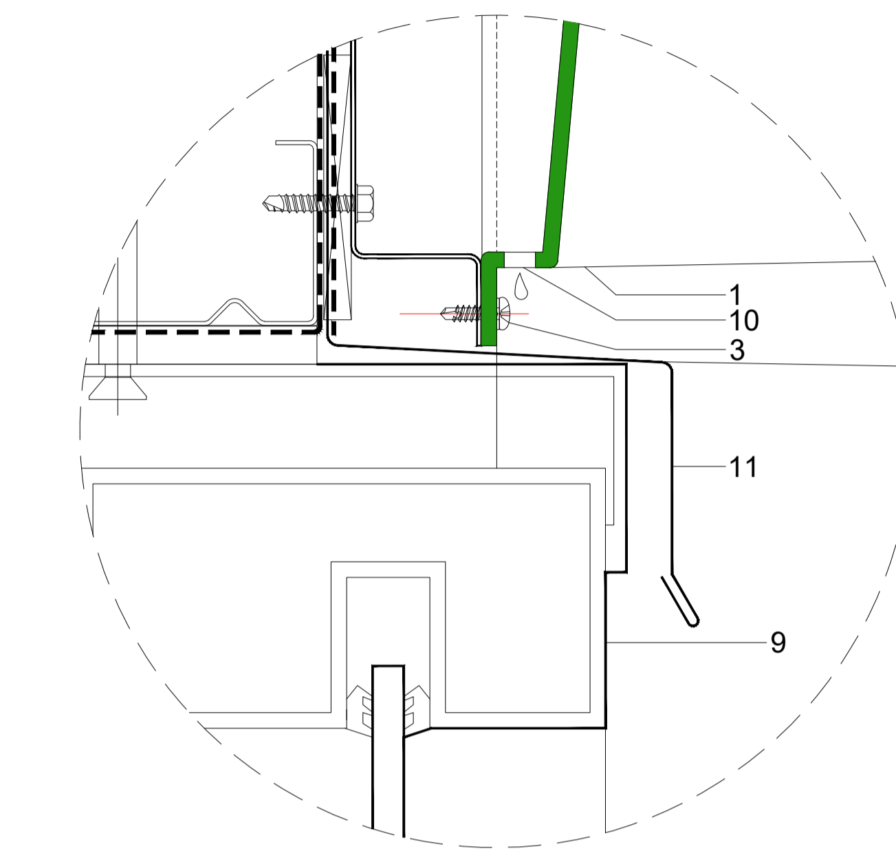
TEGO® Window Head Detail 1:1
